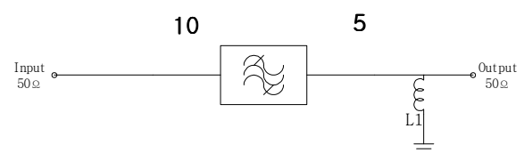
Matching Schematic
