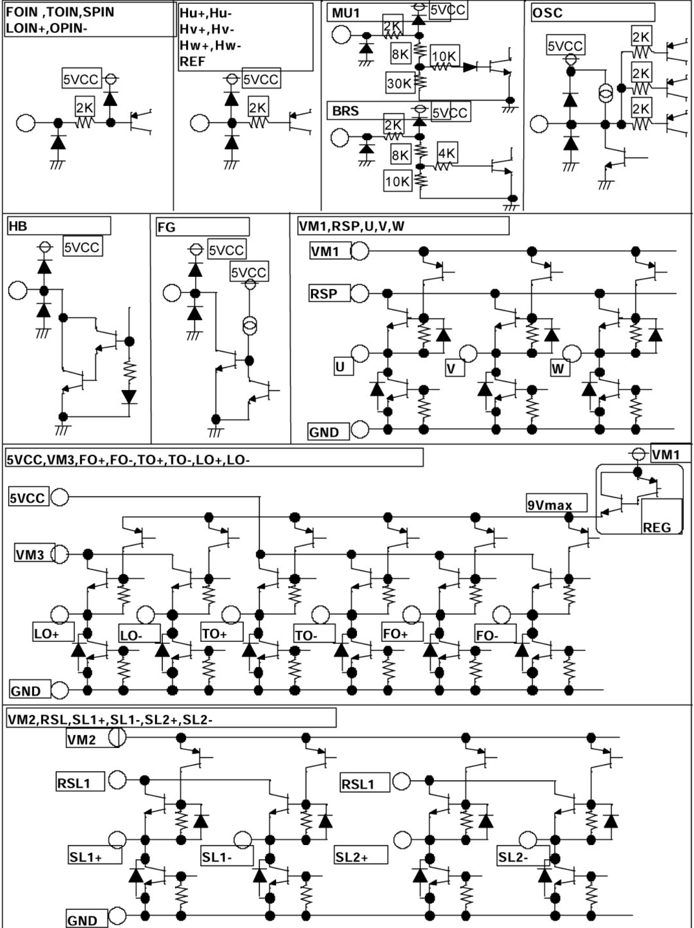
I/O circuit
