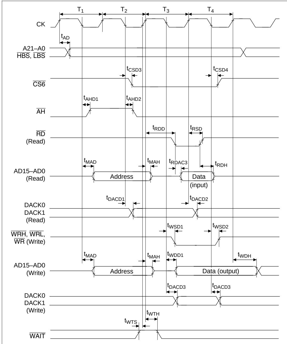
Figure 20.32 Address/Data Multiplex I/O Bus Cycle
