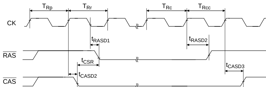
Figure 20.31 Self-Refresh
