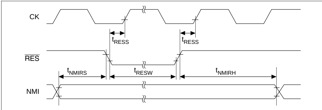
Figure 20.4 Reset Input Timing
