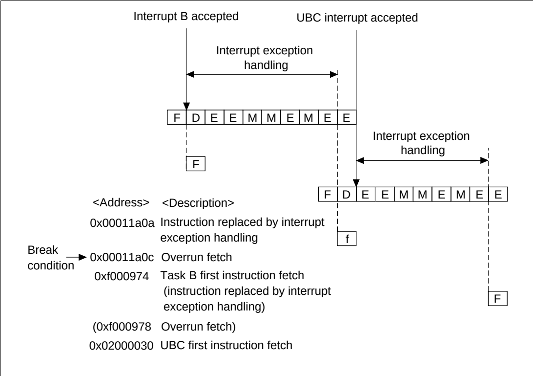
Figure 6.3 UBC Operation
