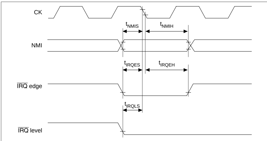
Figure 20.49 Interrupt Signal Input Timing
