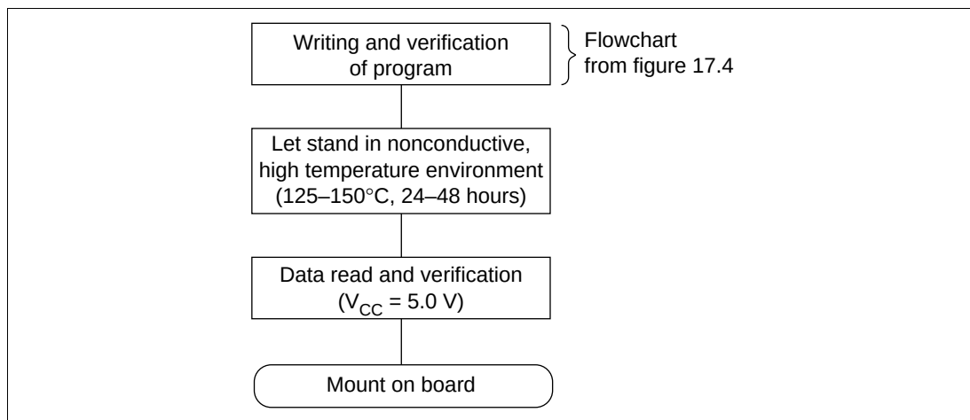
Figure 17.6 Screening Flow
