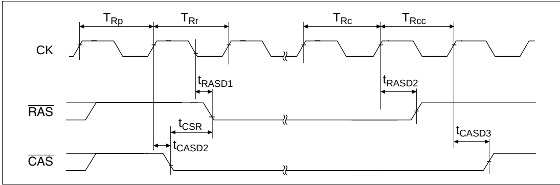
Figure 20.62 Self-Refresh
