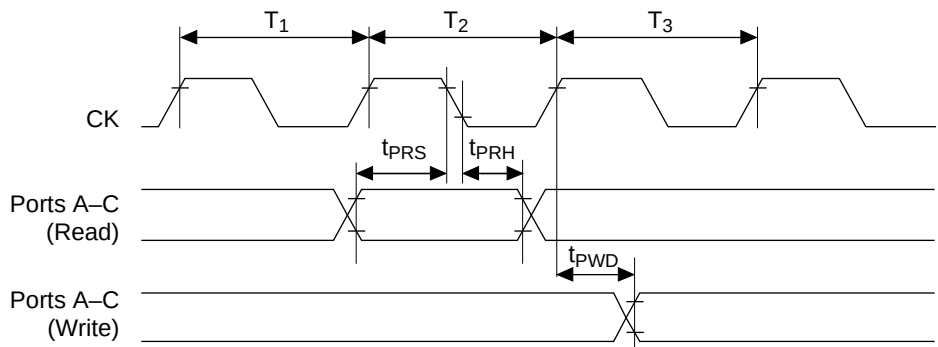
Figure 20.38 Programmable Timing Pattern Controller Output Timing
