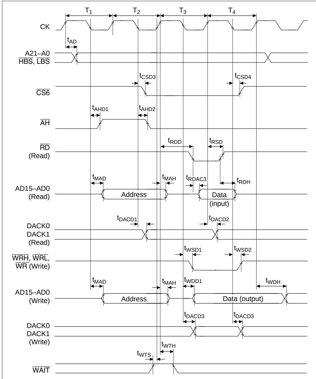
Figure 20.63 Address/Data Multiplex I/O Bus Cycle
