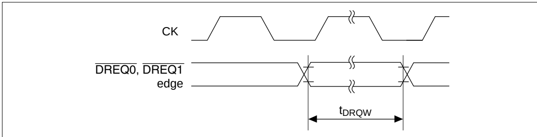
Figure 20.66 \overline{DREQ0} , \overline{DREQ1} Input Timing (2)
