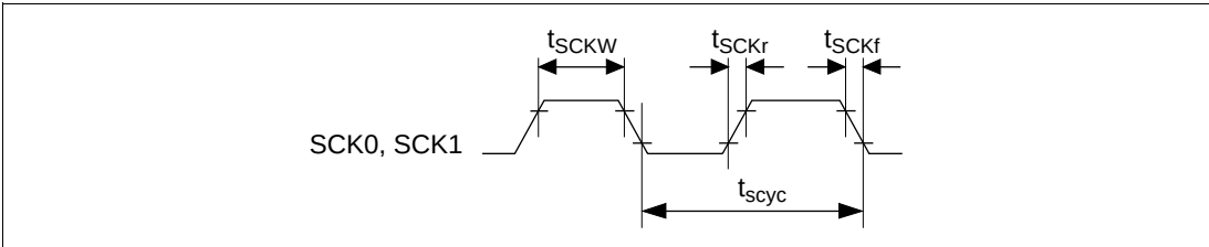
Figure 20.71 Input Clock Timing
