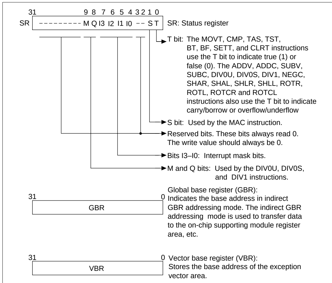
Figure 2.2 Control Registers
