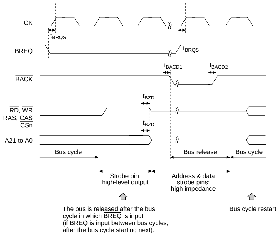
Figure 8.47 Bus Release Procedure
