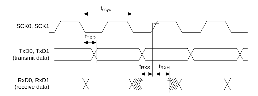
Figure 20.72 SCI I/O Timing (Synchronous Mode)
