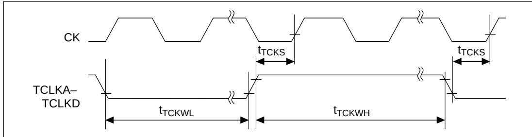
Figure 20.68 ITU Clock Input Timing
