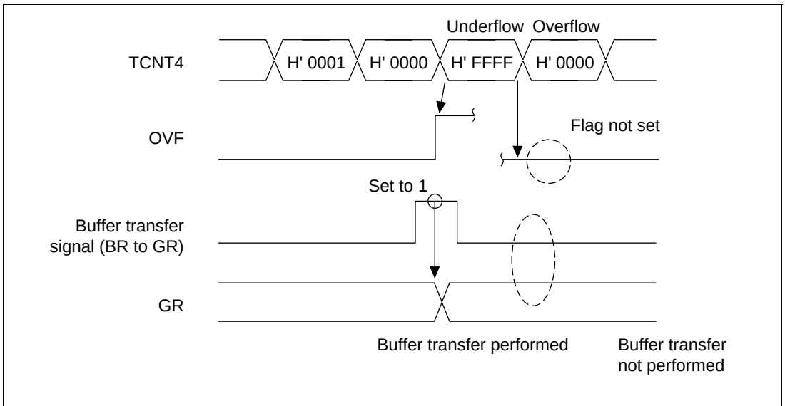
Figure 10.37 Undershoot Timing
