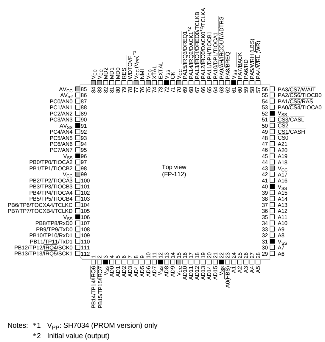
Figure 1.2 Pin Arrangement (FP-112)
