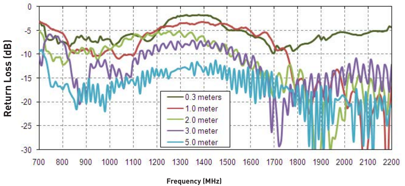
Figure 2. Return Loss of the MA104 antenna in free space
