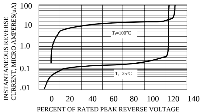
FIG. 4-TYPICAL REVERSE CHARACTERISTICS
