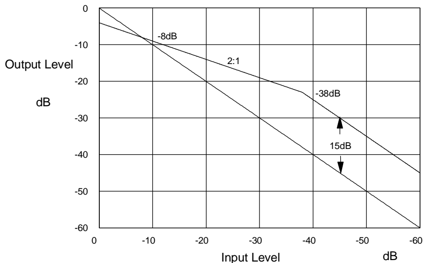
Figure 18. Compander Characteristic
