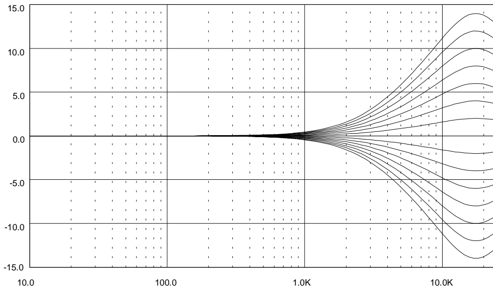
Figure 11. Treble Control @ fC = 17.5kHz
