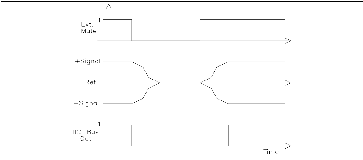
Figure 5. Softmute-Timing
