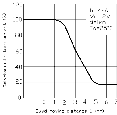
Fig.8 Relative Collector Current vs. Card Moving Distance (l)
