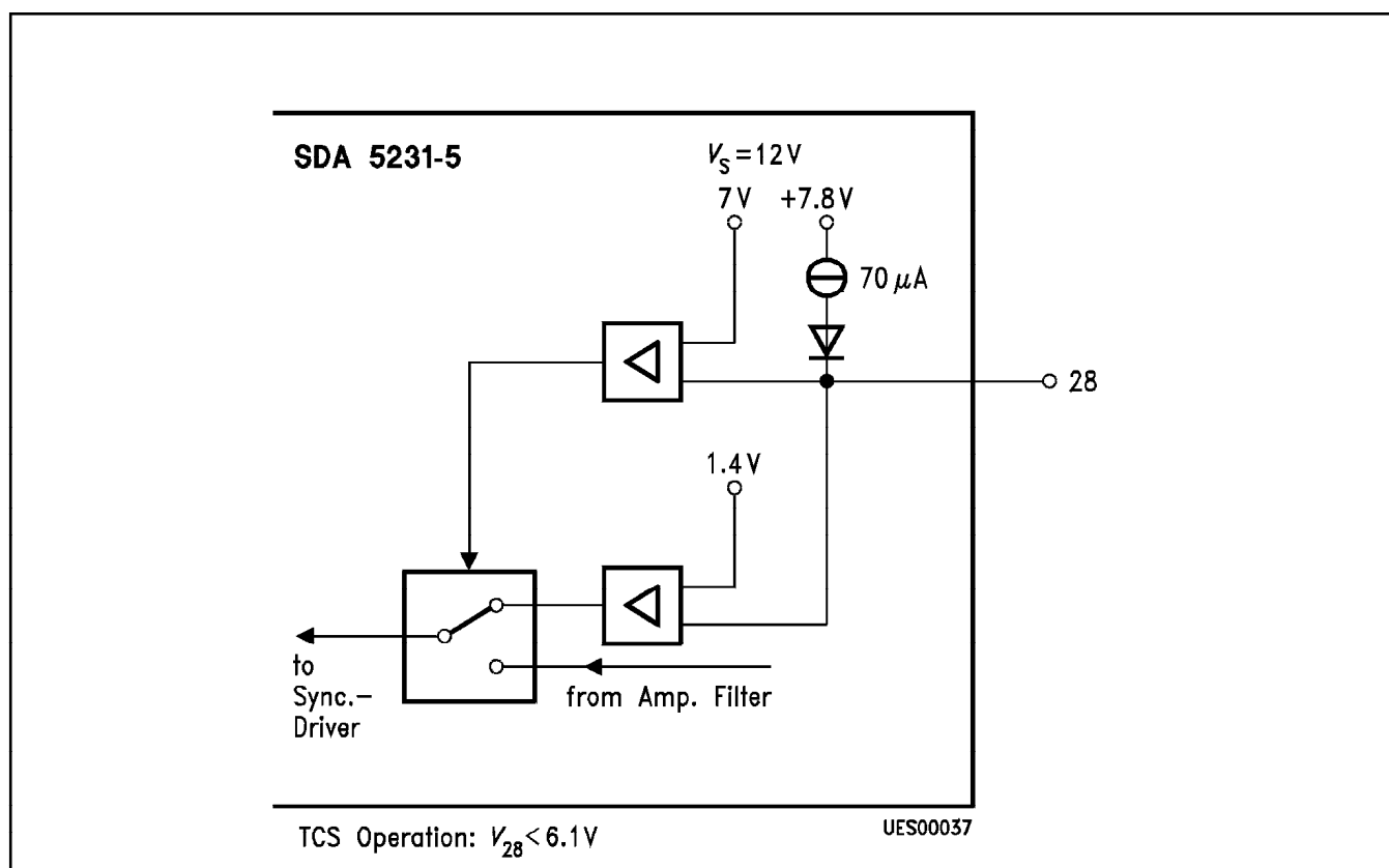
Pin 28
