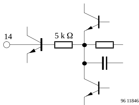
Figure 15. De-emphasis (Pin 14)
