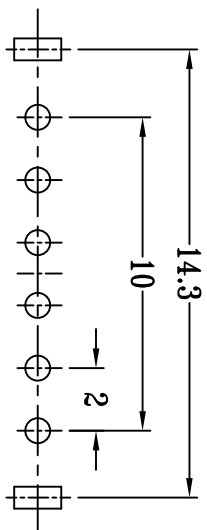
P.C.B LAYOUT BOTTOM VIEW
