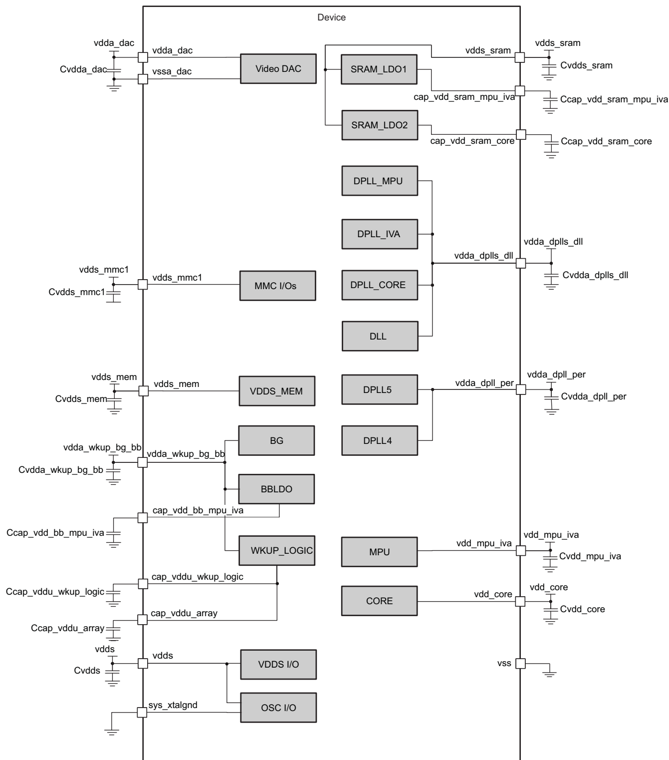
Figure 3-1. External Capacitors
