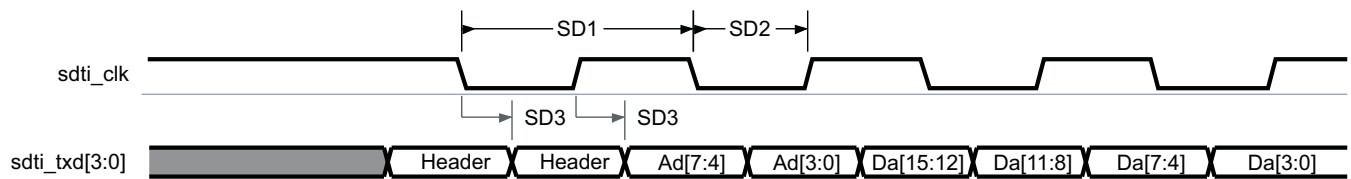
Figure 6-76. SDTI—Dual-Edge Mode
