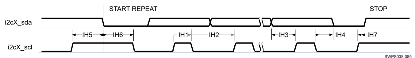
Figure 6-50. I²C—High-Speed Mode
