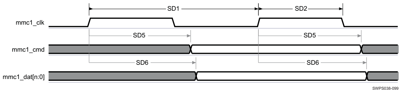
Figure 6-64. MMC1 Interface—Standard SD Mode—Data/Command Transmit
