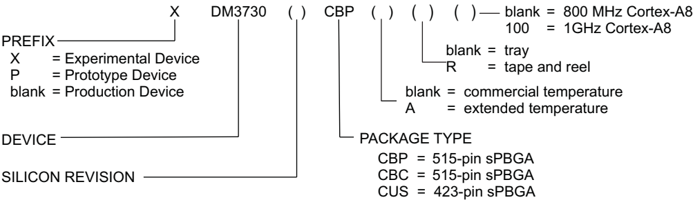
Figure 7-1. Device Nomenclature
