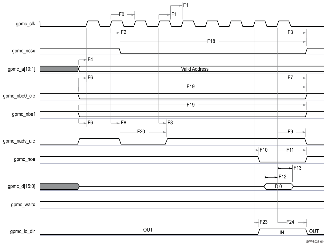
Figure 6-2. GPMC/NOR Flash—Synchronous Single Read—(GpmcFCLKDivider = 0)
