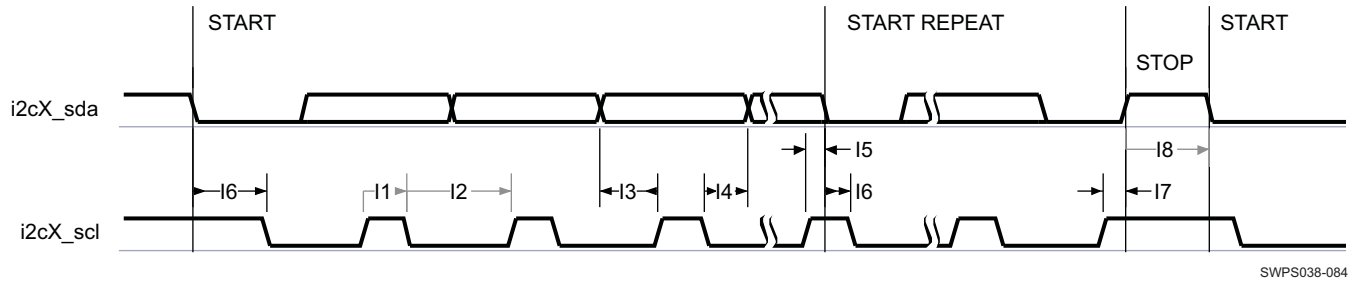
Figure 6-49. I²C—Standard and Fast Modes
