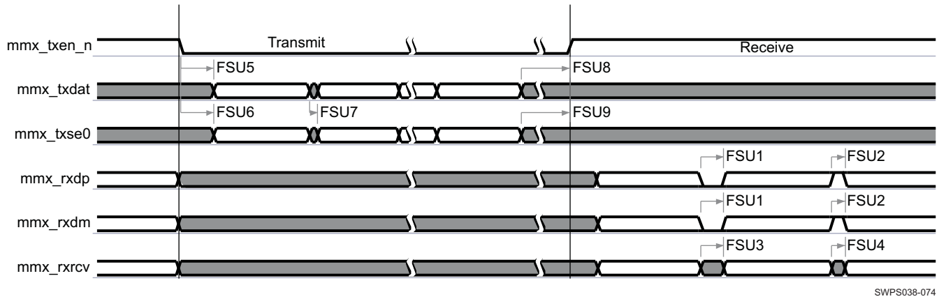
Figure 6-44. LS- / FS-USB—Unidirectional Standard 6-Pin Mode
