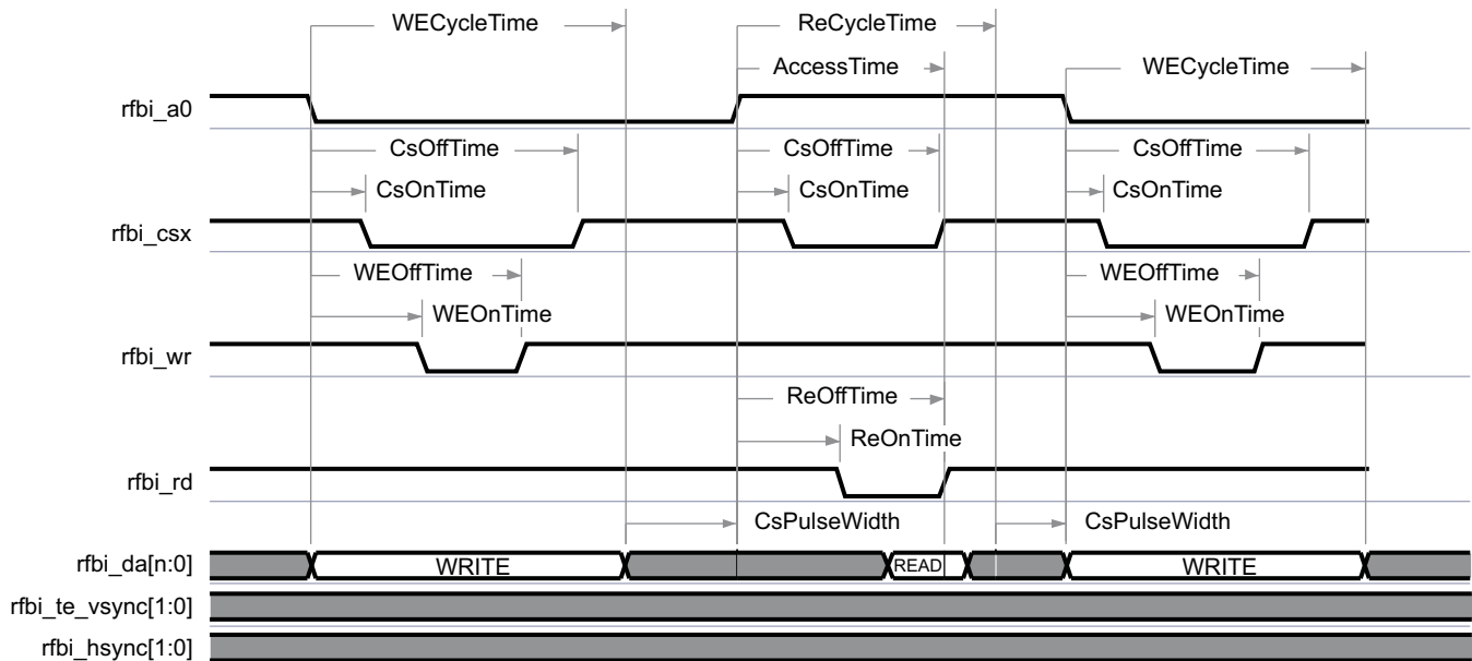
Figure 6-29. DSS—RFBI Mode—MIPI DBI 2.0 —LCD Panel—Command / Data Read
