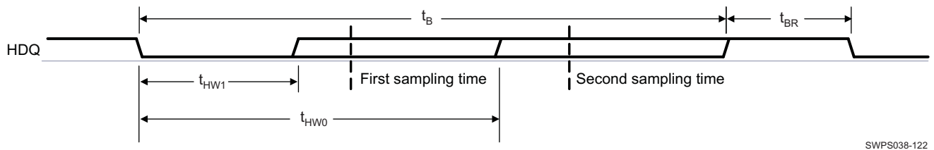
Figure 6-52. HDQ Break Detection— HDQ Interface Reading Slave
