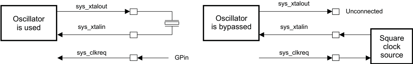
Figure 4-1. Clock Interface
