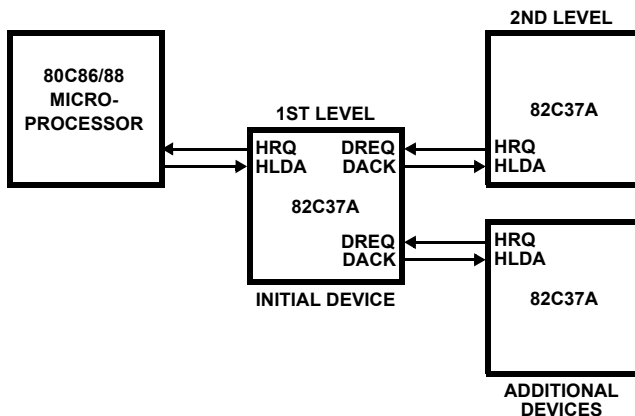
FIGURE 3. CASCADED 82C37As
