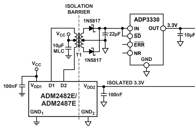
Figure 34. Applications Diagram
