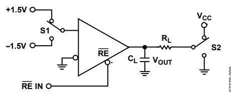
Figure 24. Receiver Enable/Disable
