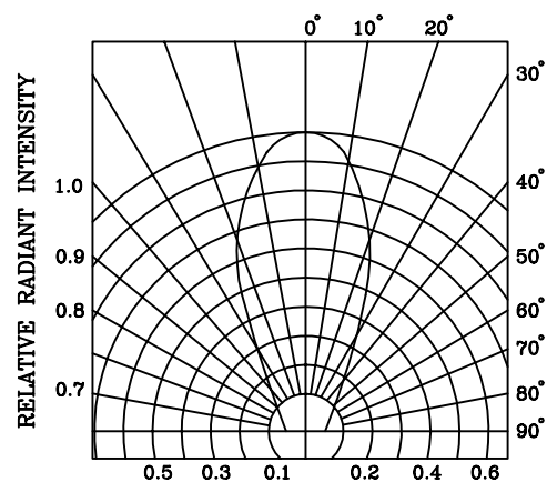
RADIATION DIAGRAM
