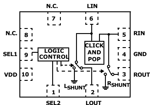
ISL54406 (10 Ld 1.8x1.4 \mu TQFN) TOP VIEW
