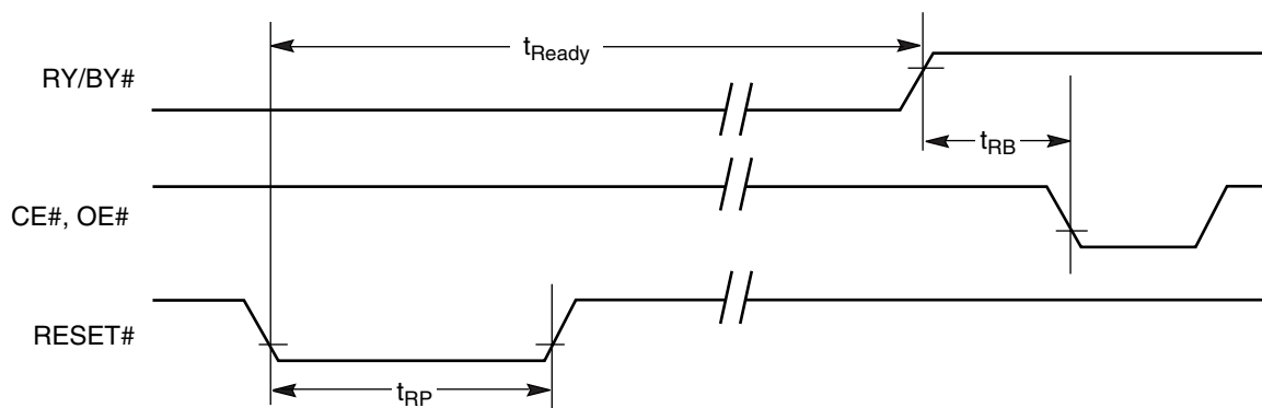
Figure 16. Reset Timings
