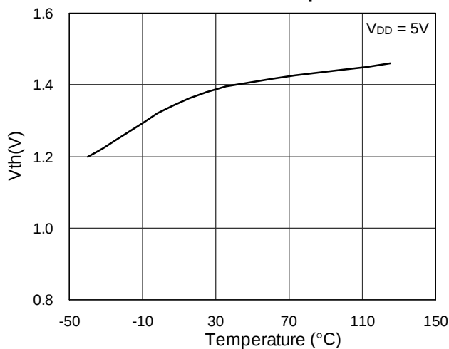
Tri-State V_{th} vs Temperature
