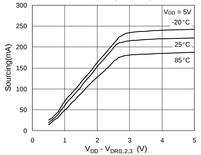
Driver Sourcing vs Drop Out
