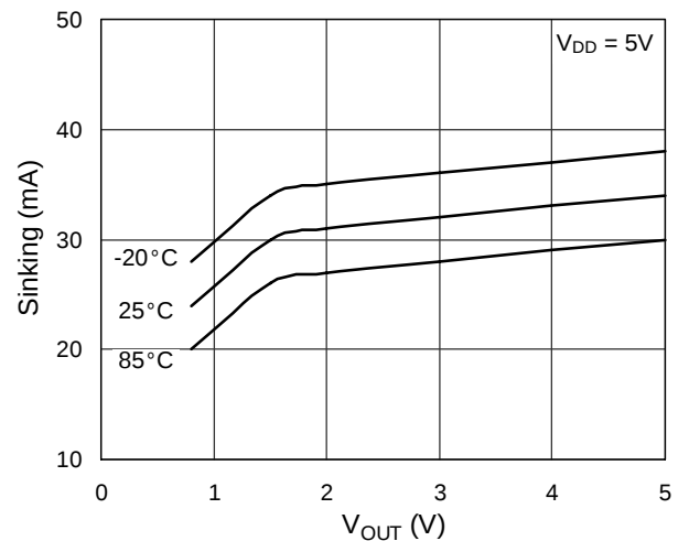
Driver Sinking vs V_{OUT}
