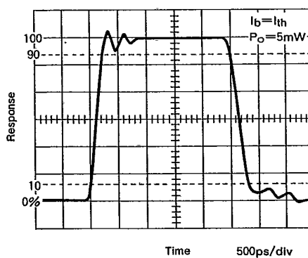
Fig. 9 Pulse response waveform
