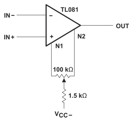
Figure 7-4. Test Figure 4
