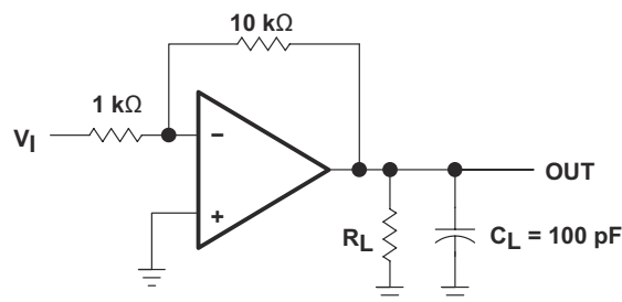
Figure 7-2. Test Figure 2
