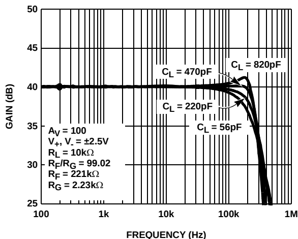
FIGURE 5. EL8170 FREQUENCY RESPONSE vs C_{LOAD}
