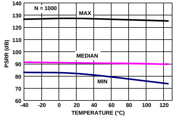
FIGURE 28. EL8173 PSRR vs TEMPERATURE, V_+ , V_- = \pm 1.2V TO \pm 2.5V
