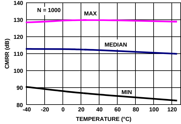
FIGURE 26. EL8173 CMRR vs TEMPERATURE, V_{CM} = +2.5V TO -2.5V , V_+ , V_- = \pm 2.5V
