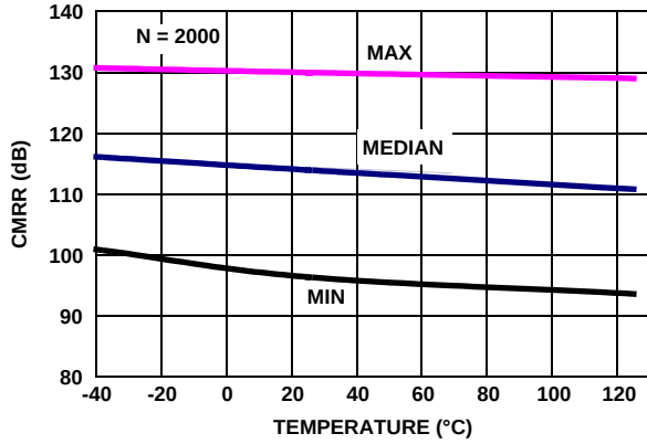
FIGURE 25. EL8170 CMRR vs TEMPERATURE, V_{CM} = +2.5V TO -2.5V , V_+ , V_- = \pm 2.5V
