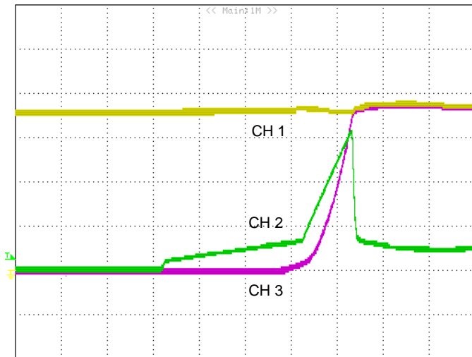
Figure 1: Input voltage turn-on threshold (2mS/div): CH1: Vin (VRTN_AF reference to -48V_AF, 10V/div). CH2: lin (-48V_AF, 2A/div). CH3: VRTN_OUT reference to -48V_OUT (10V/div).
