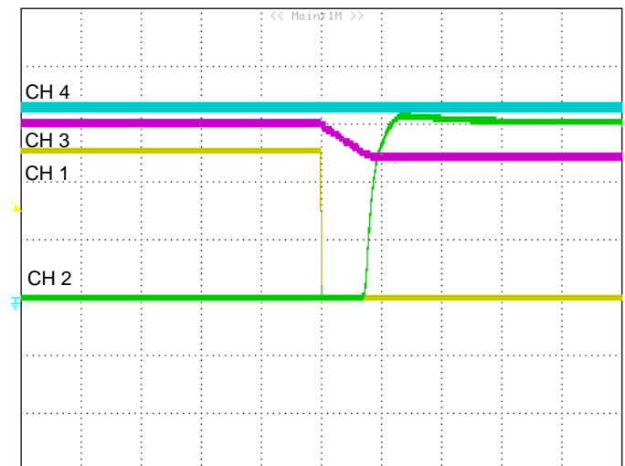
Figure 4: Oring for one feed loss (500µS/div): CH1: linA (2A/div) CH2: linB (2A/div). CH3: VRTN_OUT reference to -48V_OUT (10V/div). CH4: VMGMT_PWR (1V/div).
