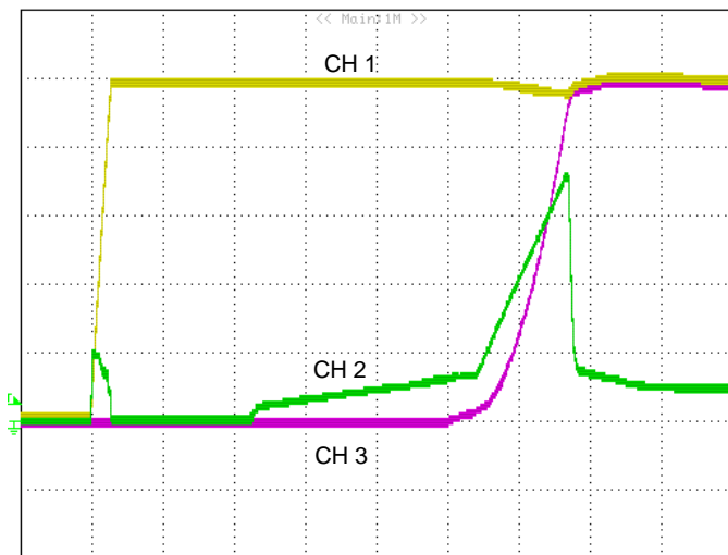
Figure 3: Inrush current (2mS/div): CH1: Vin (VRTN_AF reference to -48V_AF, 10V/div). CH2: lin (-48V_AF, 2A/div). CH3: VRTN_OUT reference to -48V_OUT (10V/div).
