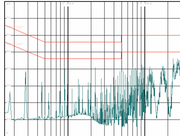
Figure 11: EMI test result with Q48SH12025NRFA:
