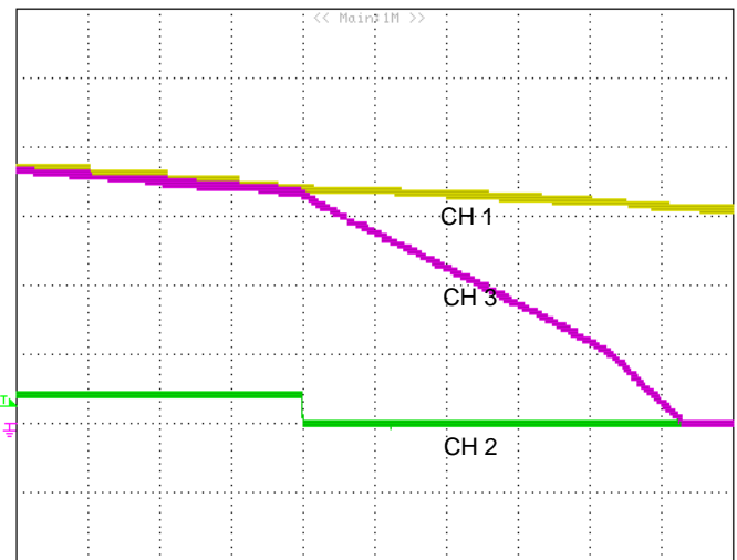
Figure 2: Input voltage turn-off threshold (2mS/div): CH1: Vin (VRTN_AF reference to -48V_AF, 10V/div). CH2: lin (-48V_AF, 2A/div). CH3: VRTN_OUT reference to -48V_OUT (10V/div).
