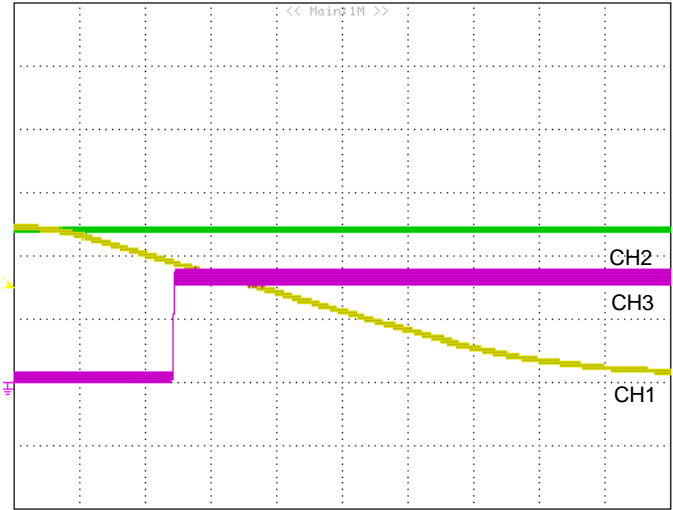
Figure 6: -48V_ALARM with loss of Feed (20mS/div): CH1: VinA (VRTN_AF reference to -48V_AF, 20V/div). CH2: VinB (VRTN_BF reference to -48V_BF, 20V/div). CH3: -48V_ALARM (2V/div)
