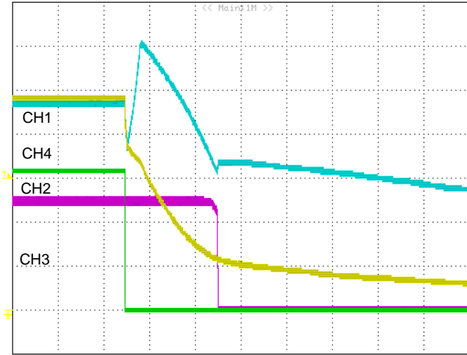
Figure 5: Hold up performance (5mS/div): CH1: Vin (VRTN_AF reference to -48V_AF, 10V/div). CH2: Iin (2A/div). CH3: 12V Vout (5V/div). CH4: VRTN_OUT reference to -48V_OUT (10V/div).
