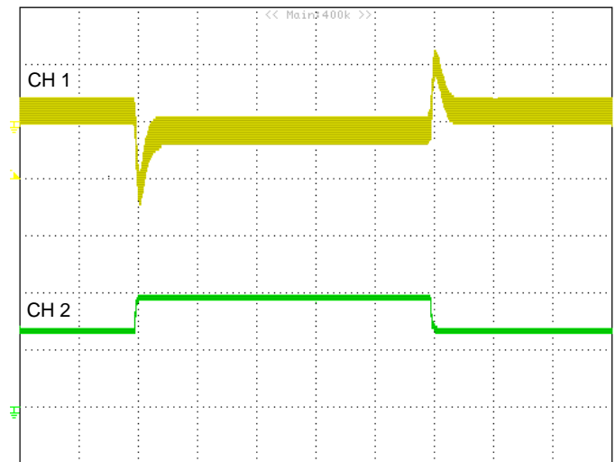
Figure 10: MGMT_PWR (3.3V) dynamic response (1mS/div):
