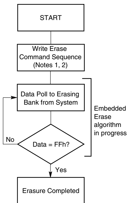
Figure 7. Erase Operation
