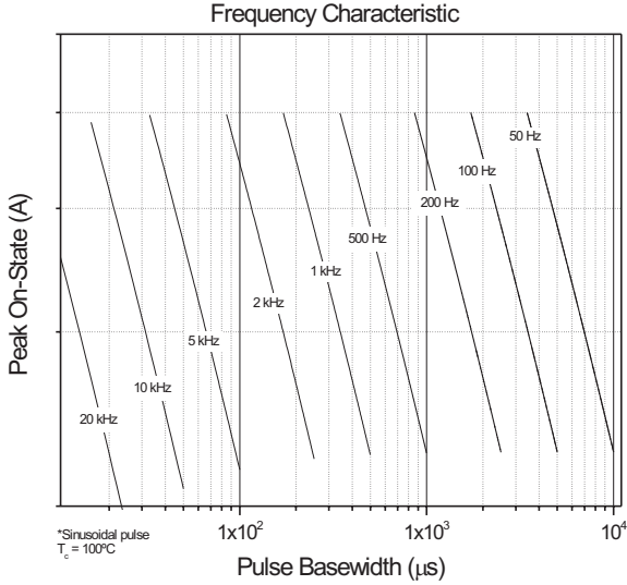
Fig. 11 - Frequency Characteristics
