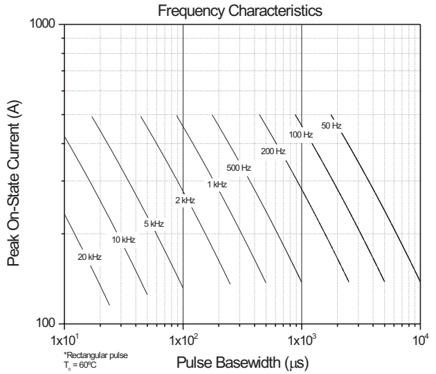
Fig. 8 - Frequency Characteristics
