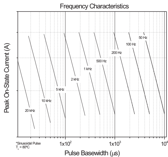
Fig. 9 - Frequency Characteristics
