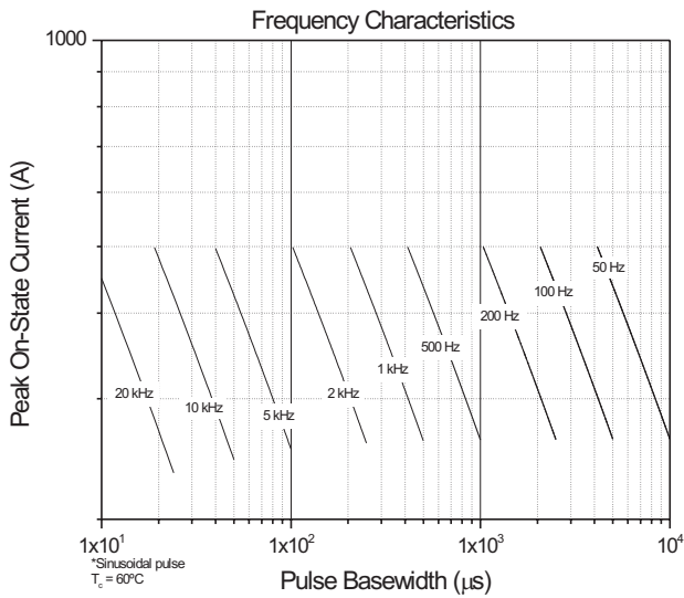
Fig. 7 - Frequency Characteristics
