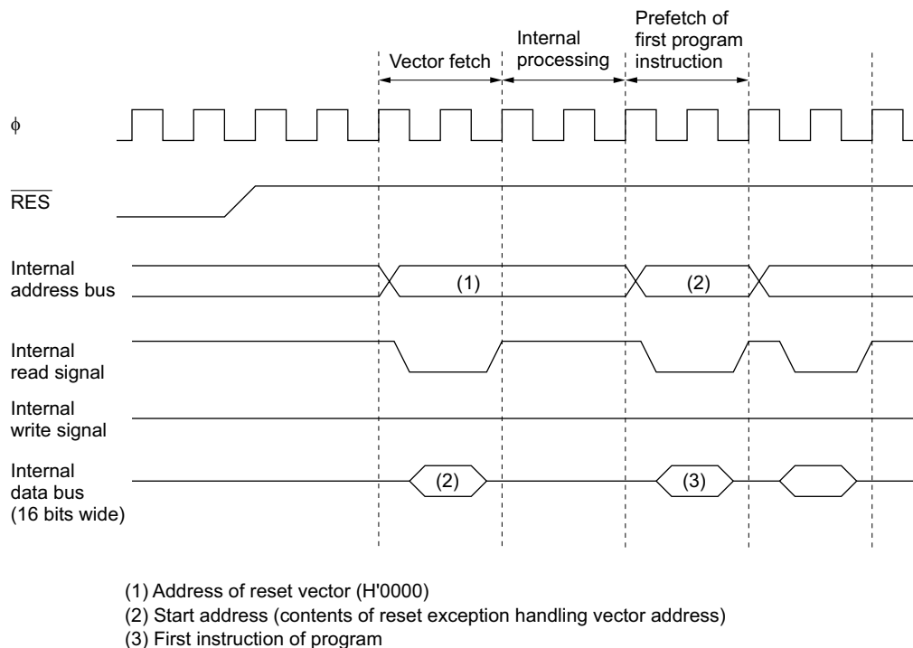
Figure 4.4 Reset Sequence (Mode 6)
