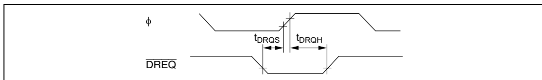
Figure 21.27 DMAC \overline{\text{DREQ}} Input Timing
