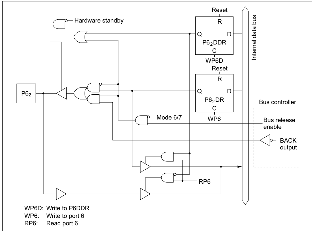
Figure C.6 (c) Port 6 Block Diagram (Pin P6 2 )
