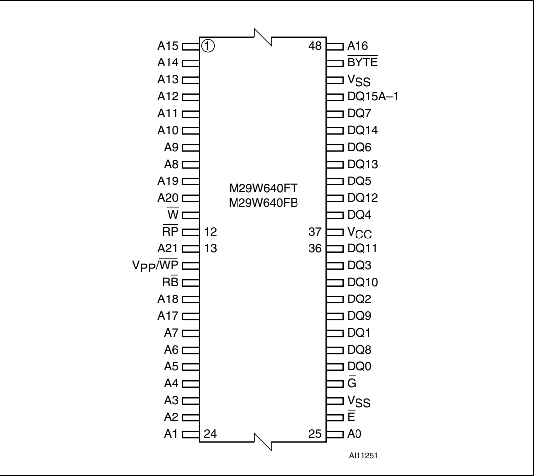
Figure 2. TSOP connections
