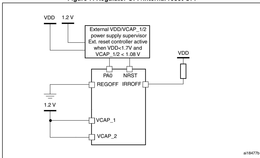
Figure 7. Regulator OFF/internal reset OFF
