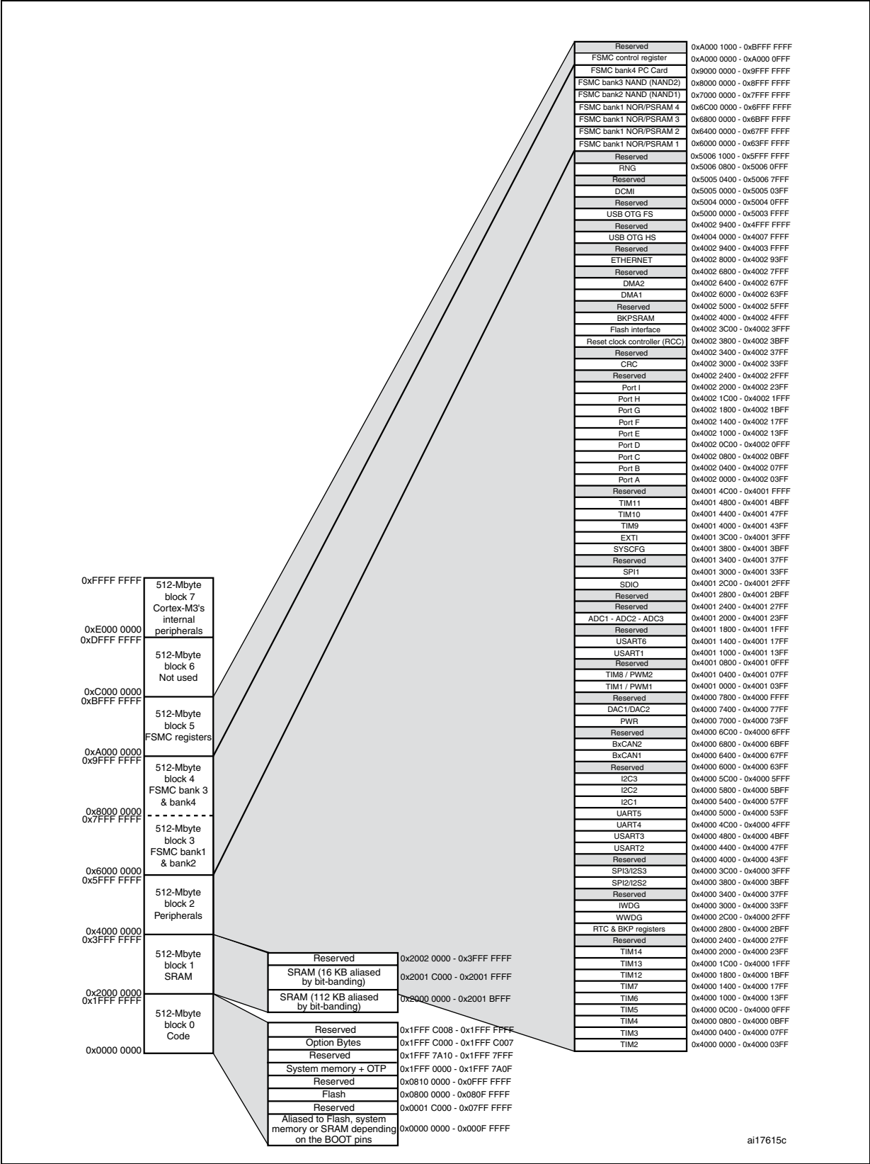
Figure 16. Memory map
