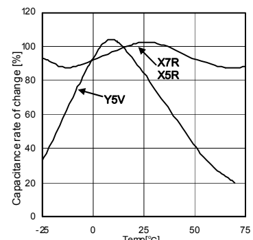
Fig.29 Capacitance vs Temperature (X5R, X7R, Y5V)
