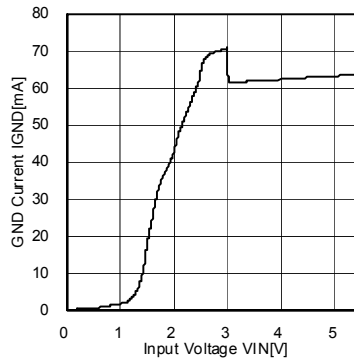
Fig.5 GND Current vs Input Voltage (BH30NB1WHFV)
