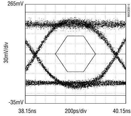
MAX3261CCJ EYE DIAGRAM (622Mbps, LOAD AT OUT- = 1300nm LASER WITH 467MHz BESSEL FILTER)*
