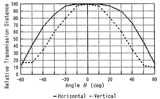
Directivity ( T_a=25^\circ\text{C} )
