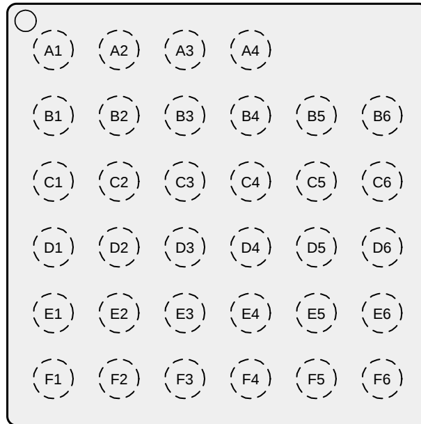
Figure 4-3. YFV (2.7-mm × 2.7-mm) Pinout, Top View
