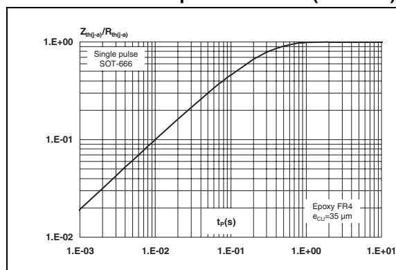
Figure 5. Relative variation of thermal impedance junction to ambient versus pulse duration (SOT-666)
