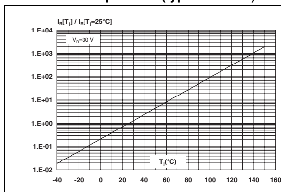
Figure 9. Relative variation of reverse leakage current versus junction temperature (typical values)
