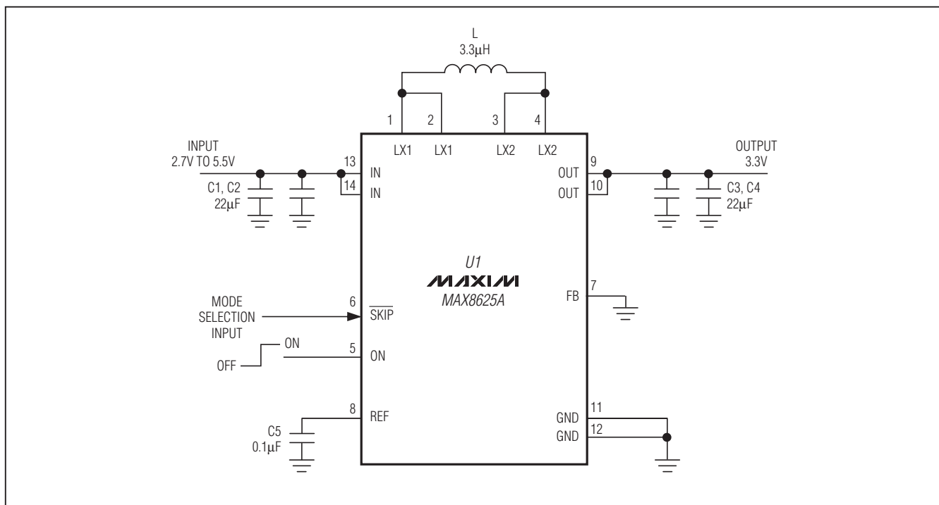
Figure 4. Typical Application Circuit (Fixed 3.3V Output)
