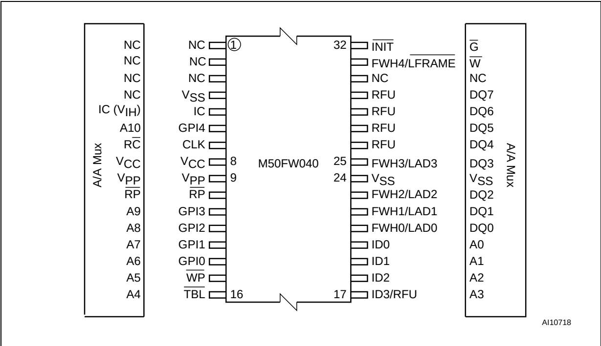
Figure 5. TSOP32 Connections
