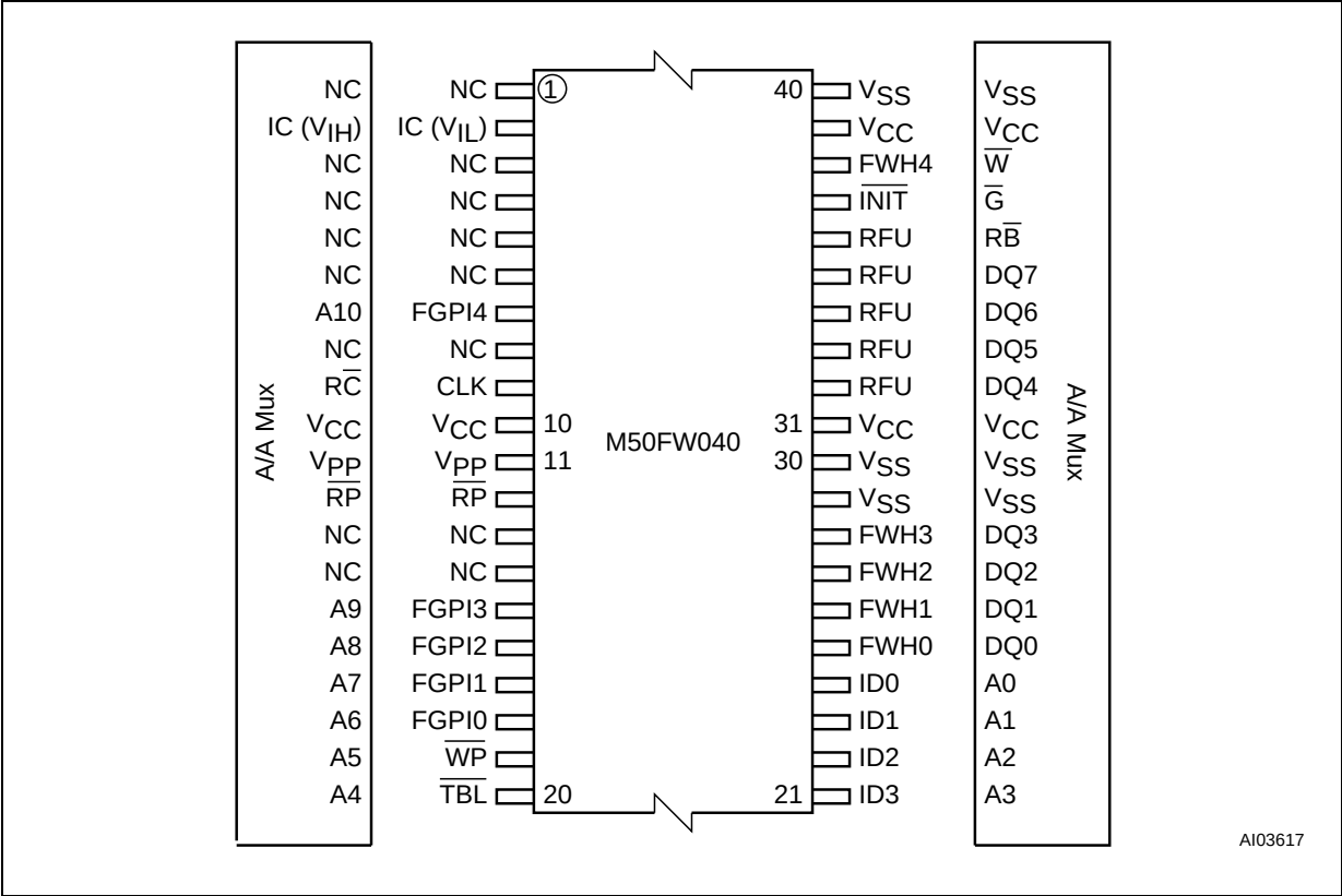
Figure 6. TSOP40 Connections
