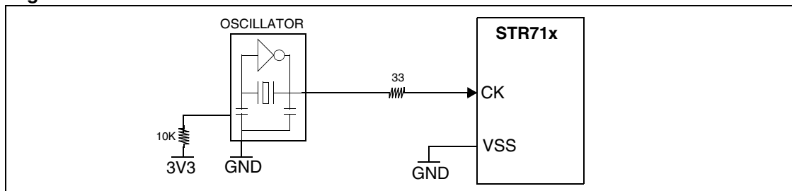
Figure 3. Main clock oscillator
