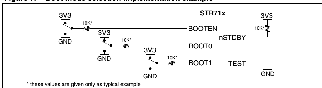
Figure 7. Boot mode selection implementation example
