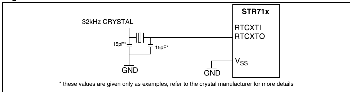
Figure 4. RTC oscillator
