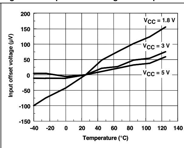
Figure 2. Input offset voltage vs. temperature
