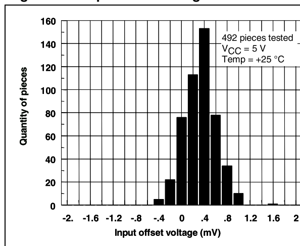
Figure 1. Input offset voltage distribution
