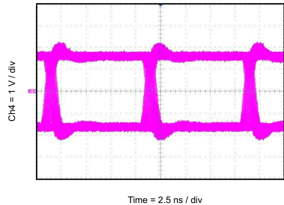
Figure 24. Eye Diagram at 100 Mbps PRBS 2 16 – 1, 3.3 V and 25°C
