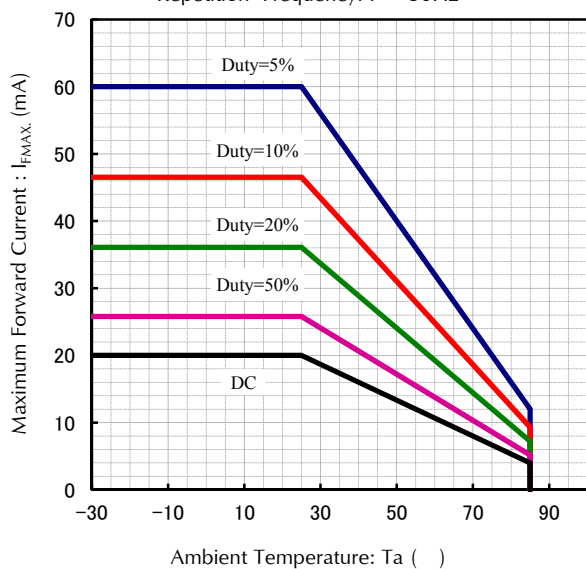
Max. Forward Current vs. Ambient Temperature
