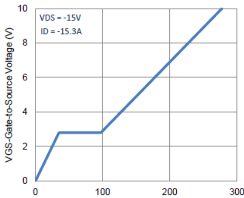
7. Gate Charge
