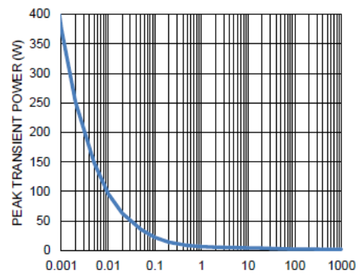
10. Single Pulse Maximum Power Dissipation
