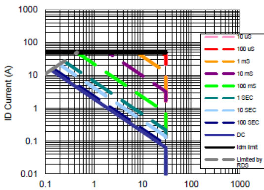
9. Safe Operating Area
