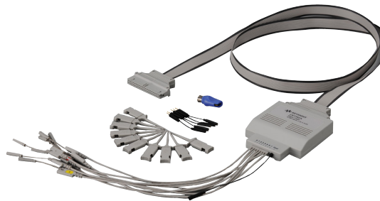
Figure 27. CX1152A 10 M \Omega Input Digital Channel
