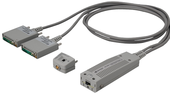
Figure 24. CX1102A Dual Channel Current Sensor (Furnished CX1203A)
