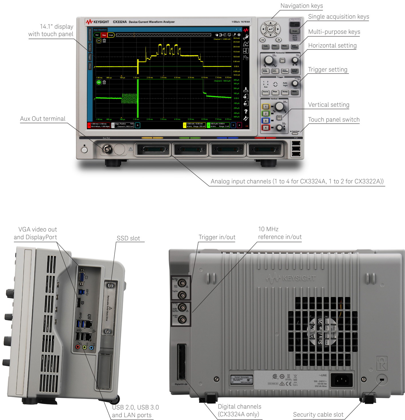
Figure 22. CX3324A front, rear and side views
