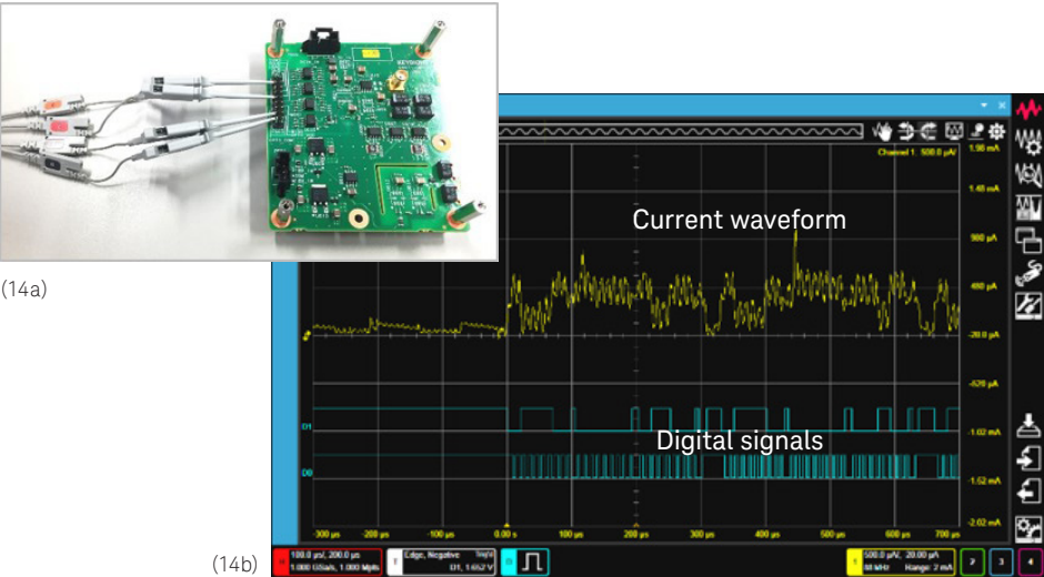
Figure 14a and 14b. Current waveform measurement and connection example using the Digital Channel
