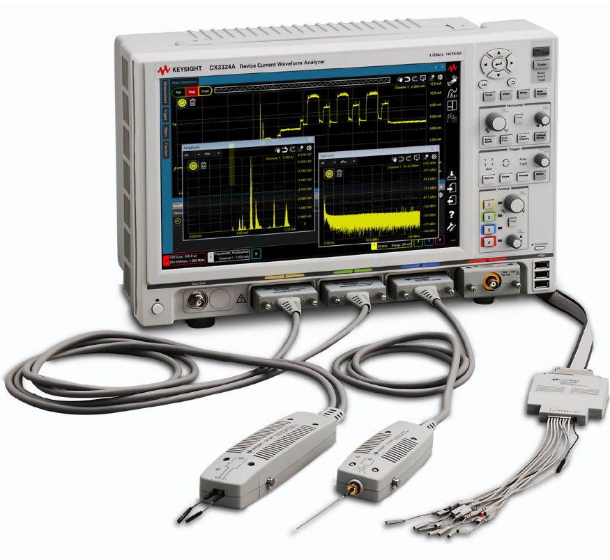
Figure 5. The CX3300's dedicated current sensors greatly suppress high frequency current noise without losing their low-burden current sensing capability. The dual channel sensor enables almost 5-decade dynamic range using the simultaneous dual range view technology.
