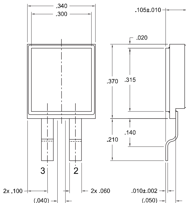
CASE OUTLINE: Cerpack (G)
