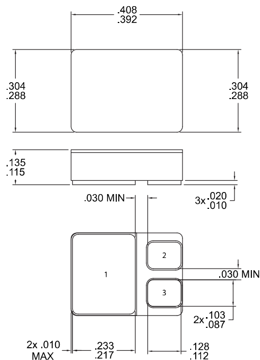
CASE OUTLINE: SMD.5 (S.5)
