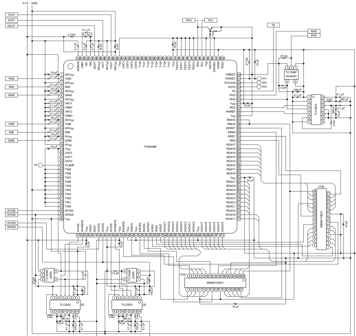
Application Circuit
