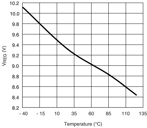
V REG vs. Temperature
