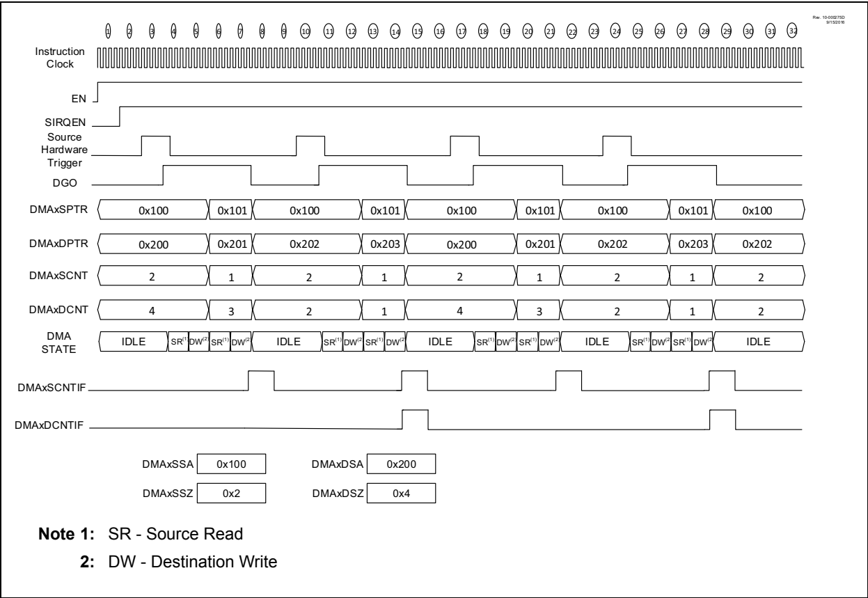
FIGURE 15-7: GPR-GPR TRANSACTIONS WITH HARDWARE TRIGGERS, SSTP, DSTP = 0
