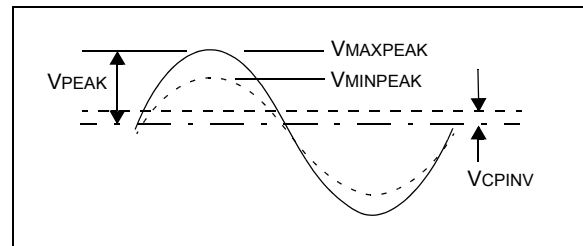
FIGURE 29-1: EXTERNAL VOLTAGE
