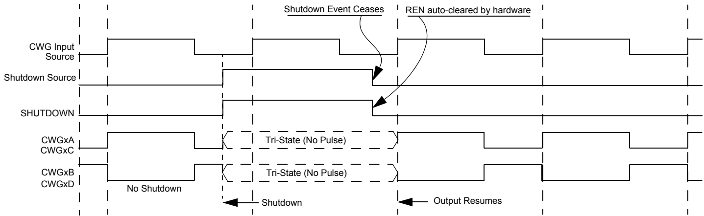
FIGURE 26-16: SHUTDOWN FUNCTIONALITY, AUTO-RESTART ENABLED (REN = 1, LSAC = 01, LSB0 = 01)
