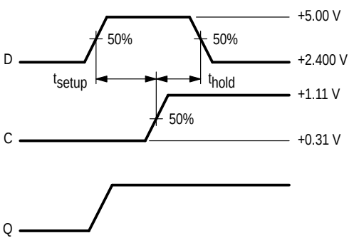
Figure 7 – TSET UP AND THOLD WAVEFORMS
