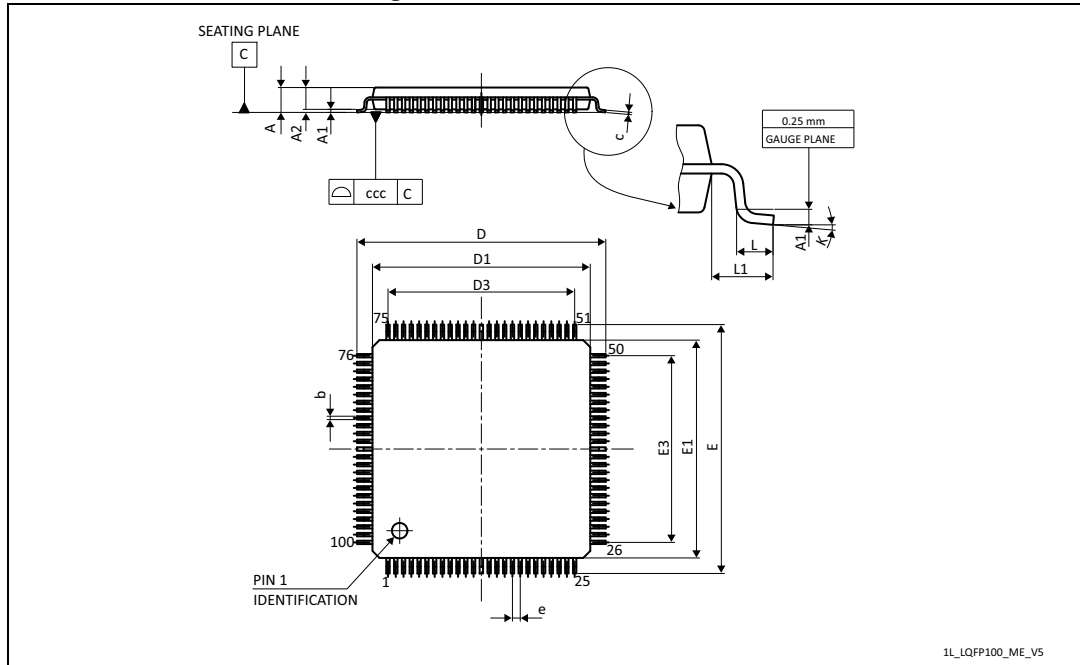
Figure 79. LQFP100 - Outline
