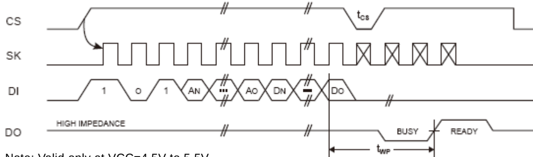
Figure 5: WRITE Timing
