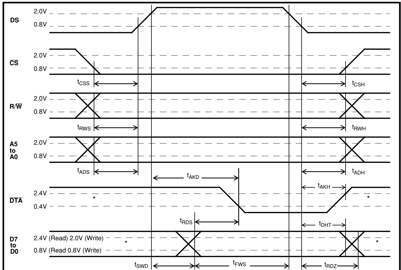
Figure 17 - Processor Bus
