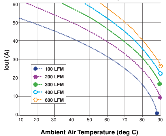
Thermal Derating Curves GHTW3V360 Heatsink Ready
