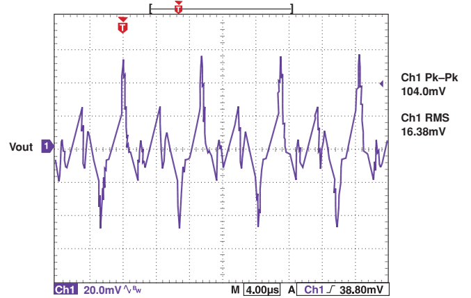
Voltage Ripple
