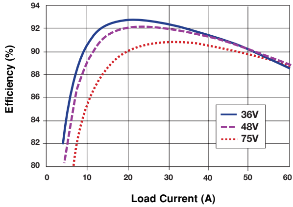
Efficiency
