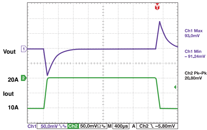
Transient Response
