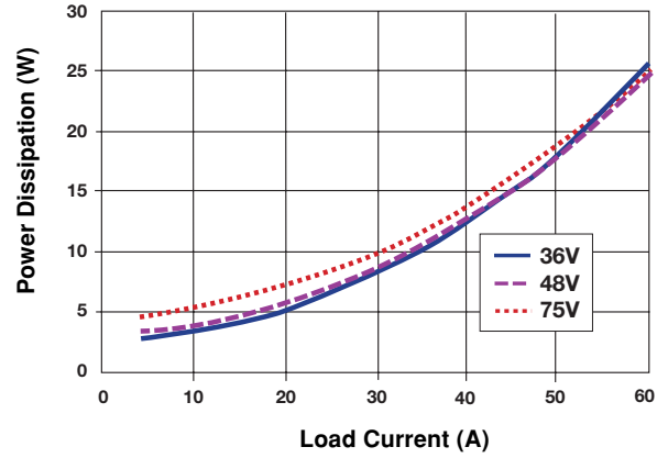
Power Dissipation
