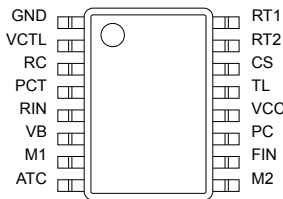
Fig.16 BA6951FS (SSOP-A16)
