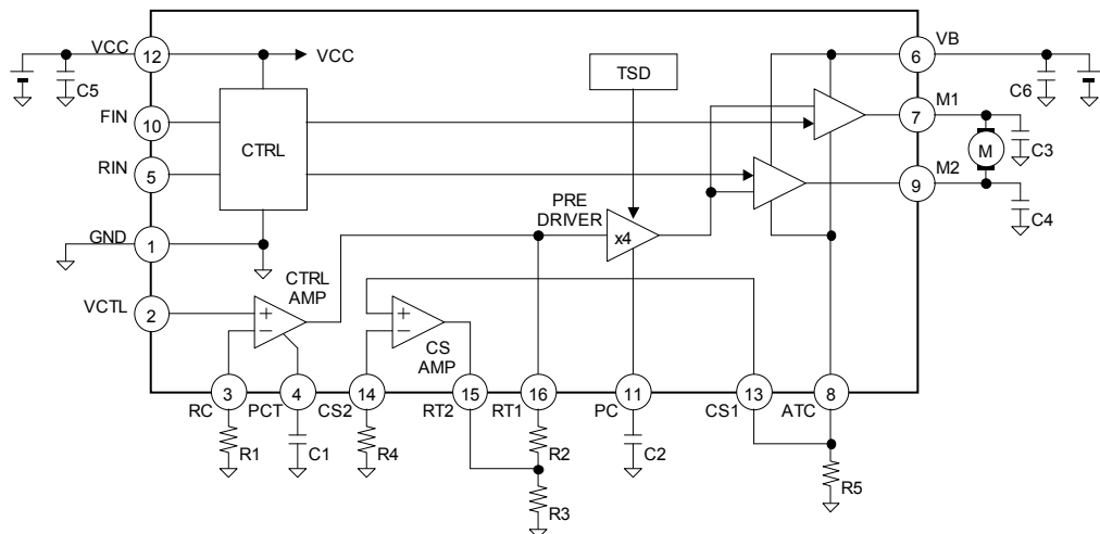
Fig.13 BA6950FS
