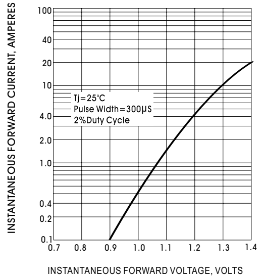
Fig. 2- TYPICAL INSTANTANEOUS FORWARD CHARACTERISTICS PER ELEMENT
